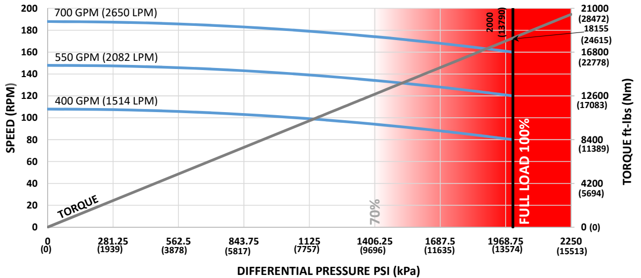
7 in (178mm) 9-10 Lobe 8.0 Stage HR
